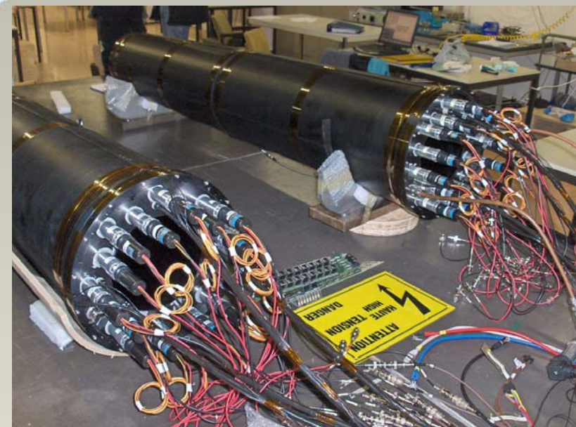
Read-out with photomultipliers and fibers
